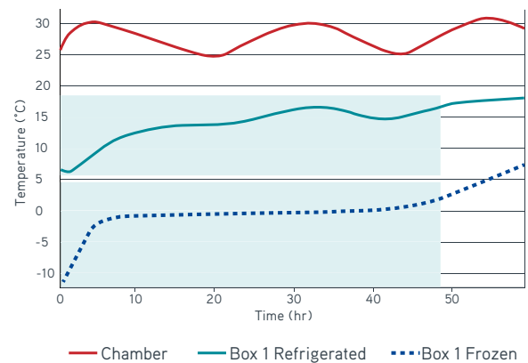
Meal Kit Delivery — ISTA 7E Hot Profile
